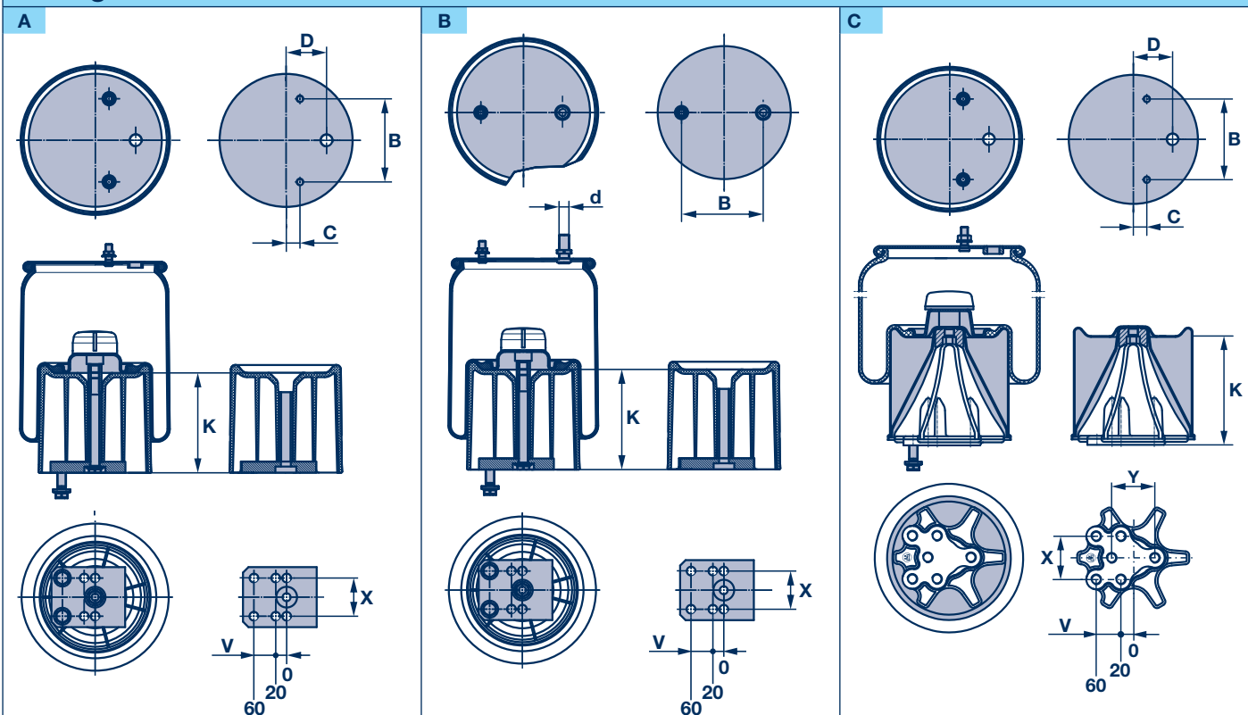
Air bag with GRP piston
